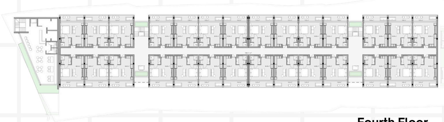
Fourth Floor
